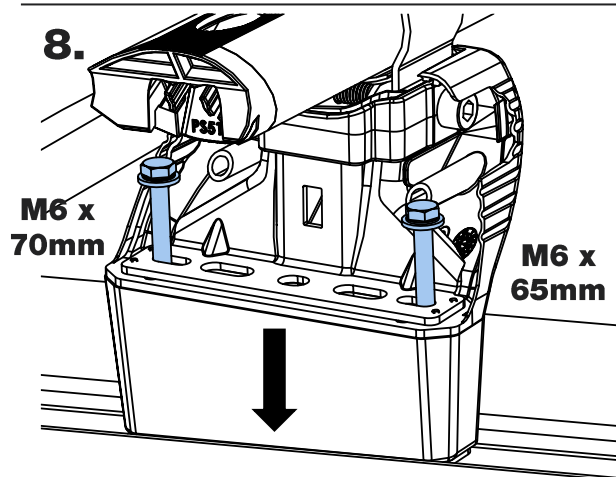
PS182 + M6 x 65/75mm
