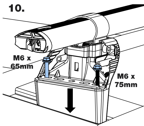
PS181 + M6 x 65/70mm
