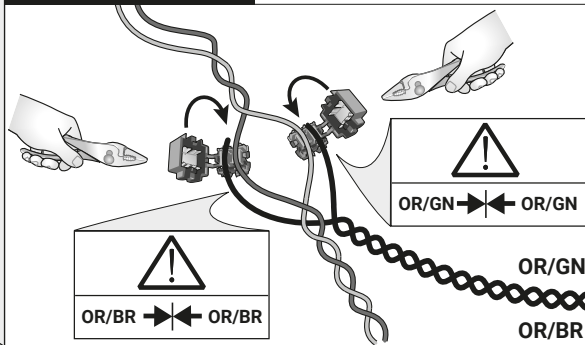
CAN-Data Wire
