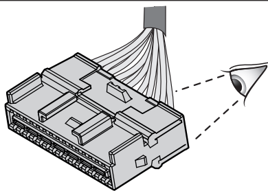
BR / 30 PIN JF01 - CAN-Bus Joint Connector
