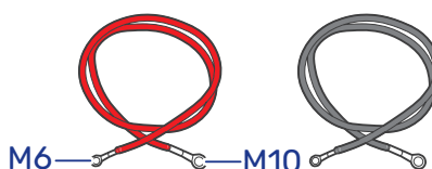
Battery Adapter Cables (8 AWG) × 2
