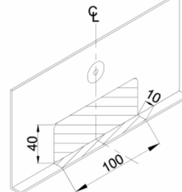
PLASTIC PANEL CUT - SEAT LEON
