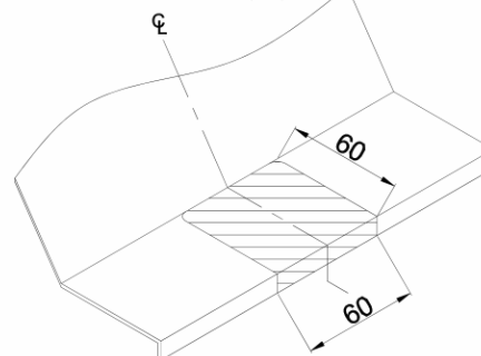
BUMPER CUT - SEAT LEON (FR)
