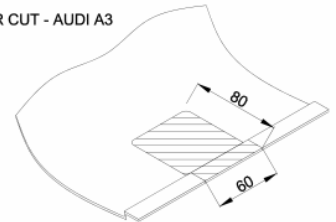
BUMPER CUT - AUDI A3
