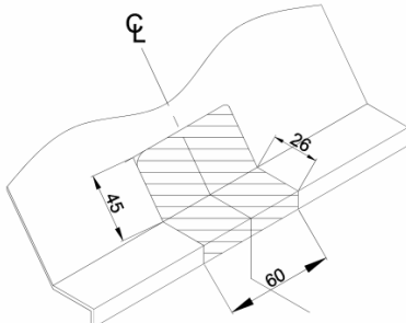
BUMPER CUT - SEAT LEON (Standard)
