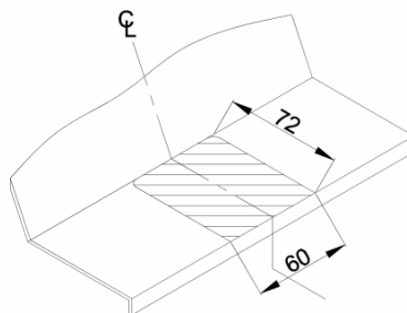
BUMPER CUT - VW GOLF VII
