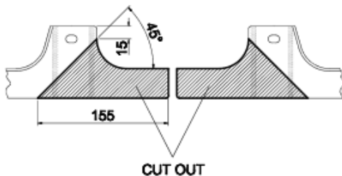
LANDCRUISER TYPE 120 L/H & R/H BUMPER SUPPORT BRACKETS
