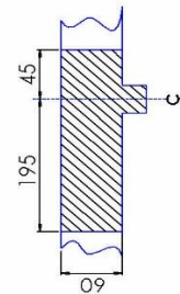
DS3 BUMPER CUT
