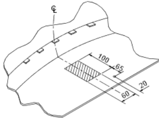
BUMPER SKIRT CUT INSIGNIA SPORT-TOURER ESTATE
