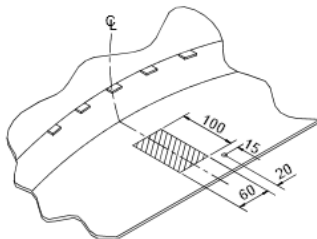
BUMPER SKIRT CUT INSIGNIA SALOON / HATCH
