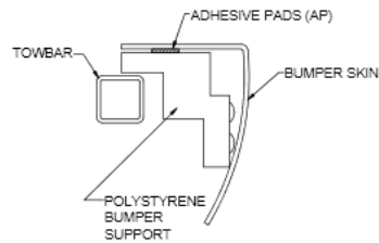
INSIGNIA SPORT TOURER BUMPER SUPPORT POSITIONING
