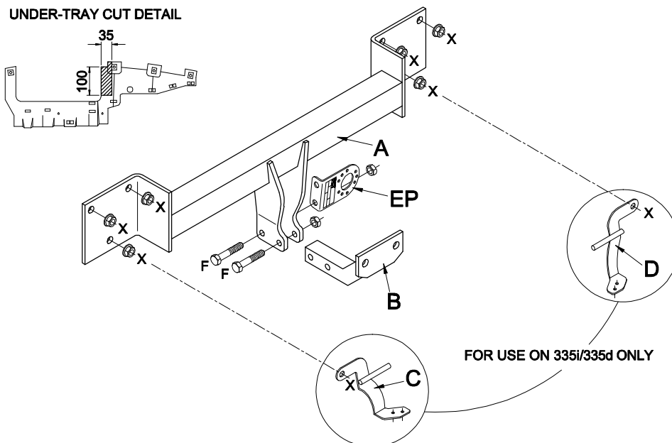
UNDER-TRAY CUT DETAIL
